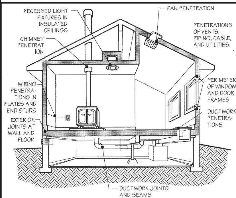
Critical areas for air leakage control. Photo courtesy of: U.S. Department of Energy, http://resourcecenter.pnl.gov/cocoon/morf/ResourceCenter/graphic/643
